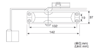
Parallel arm installation
